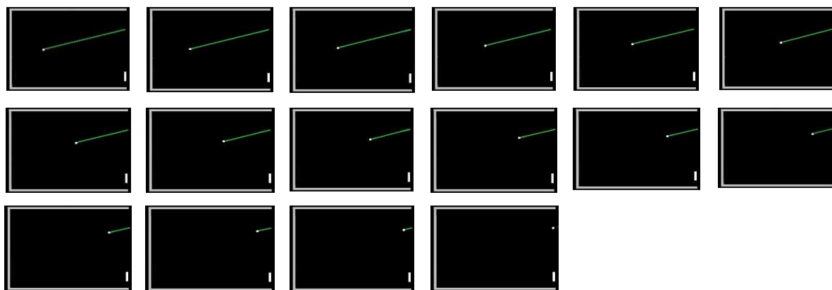
Fig.: The perception of the complex process of the tau -value approaching zero can be reduced to a very simple one-dimensional observation: the disappearance of a line. Just as a boat approaching a dock gradually reduces the visible gap between the boat and the dock, the same occurs in the incoming pong ball trajectory shape. The space between the actual position of the pong ball and the projected goal of the action trajectory shape progressively disappears.
