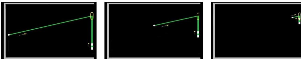
Fig.: The initial positions of the pong ball give rise to a perceptual image of a latent incoming ball trajectory shape, which in turn quickly enables the formation of a perceptual image of a potential intersection point with the movement of the paddle along an egocentric action trajectory shape. This intersection point may be represented either as a specific location or as a broader spatial zone (indicated in yellow). - The perception of the motion of both the ball and the paddle as they converge toward this intersection point involves an explanatory framework that is, at first glance, too complex to be reconciled with an ecological perspective. However, this explanation can be reduced to two simple one-dimensional phenomena. In line with the concept of the gap introduced by D.N. Lee in his tau-coupling theory, it suffices to observe how a distance disappears. Much like watching a ship approaching the dock or a long jump athlete completing the run-up towards a take-off board as the intervening space gradually reduces to zero.
