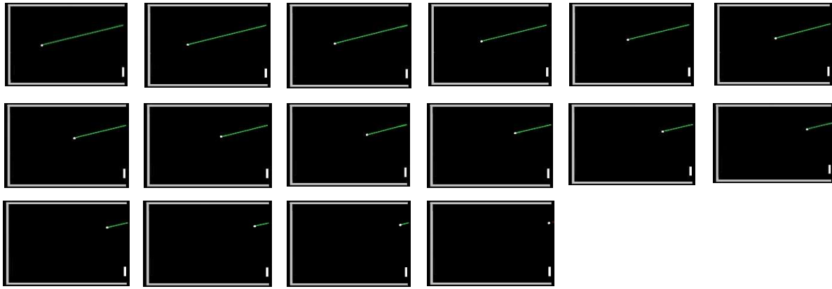
Fig.: The perception of the complex process of the tau-value approaching zero can be reduced to a very simple one-dimensional observation: the disappearance of a line. Just as a boat approaching a dock gradually reduces the visible gap between the boat and the dock, the same occurs in the incoming pong ball trajectory shape. The space between the actual position of the pong ball and the projected goal of the action trajectory shape progressively disappears.
